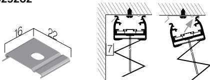
Support plafond 029202
